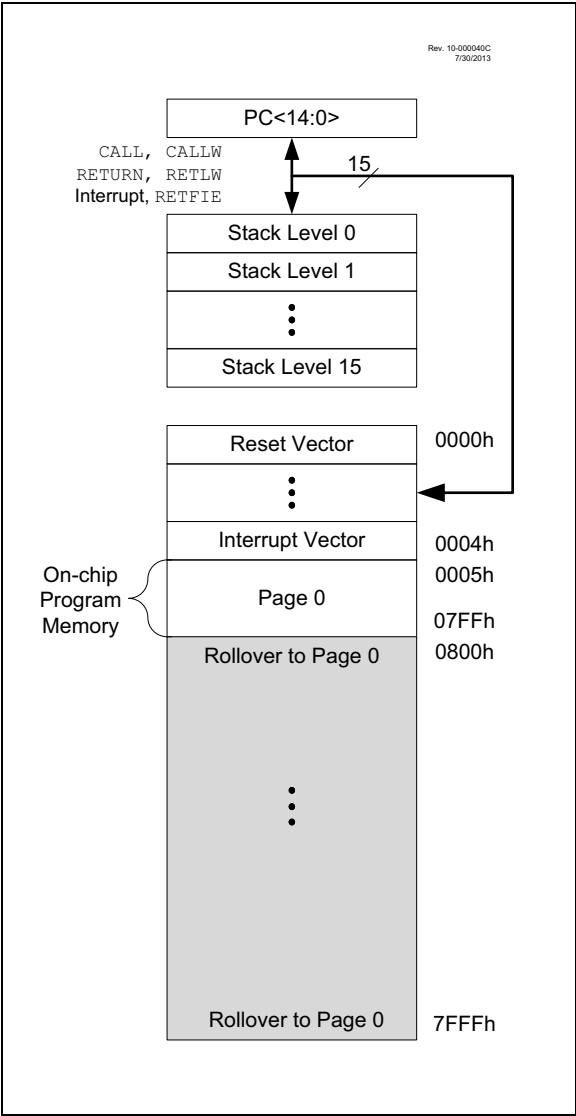
FIGURE 3-2: PROGRAM MEMORY MAP AND STACK FOR PIC12(L)F1572
