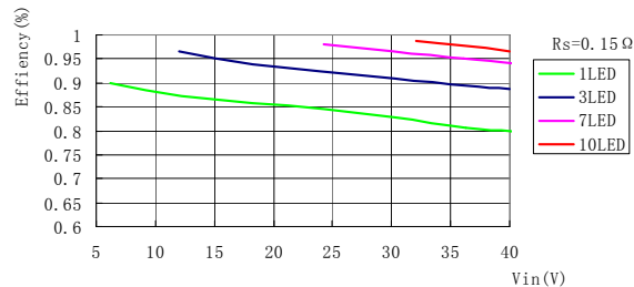
Efficiency vs. No. of LEDs L=47\mu\text{H} , R_s=0.15\Omega\text{m}
