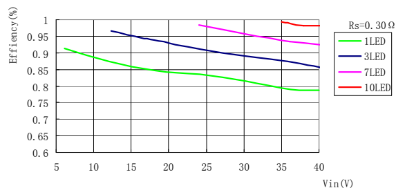
Efficiency vs. No. of LEDs L=47\mu\text{H} , R_s=0.30\Omega\text{m}
