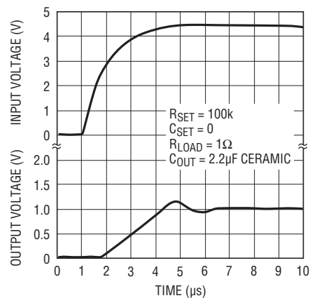
Turn-On Response
