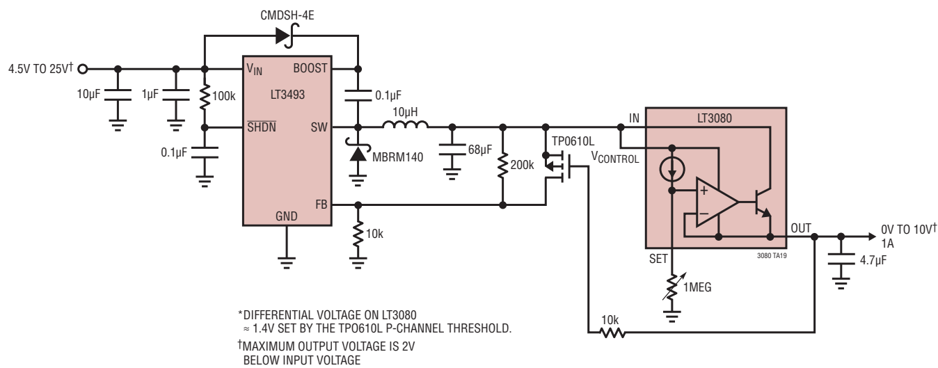
Adjustable High Efficiency Regulator*
