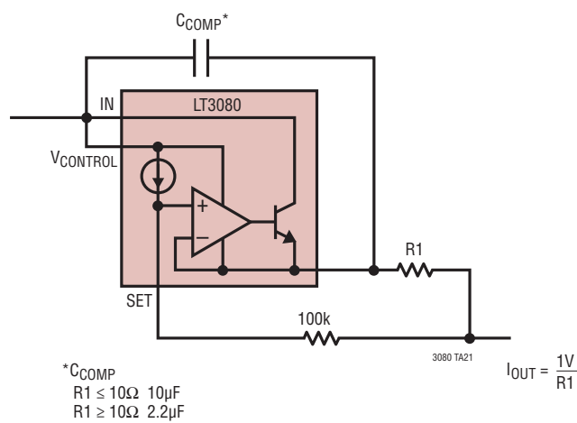
2 Terminal Current Source
