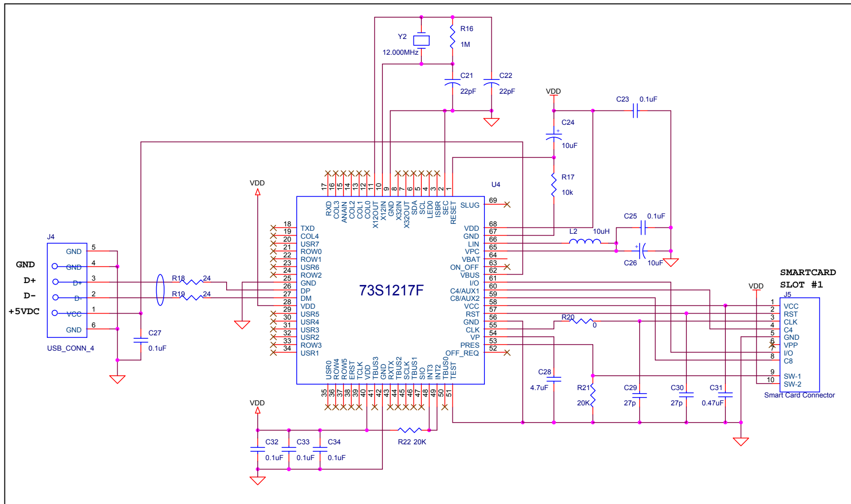
Figure 28: 73S1217F Typical Application Schematic (USB Transparent Reader and USB Key Configuration)
