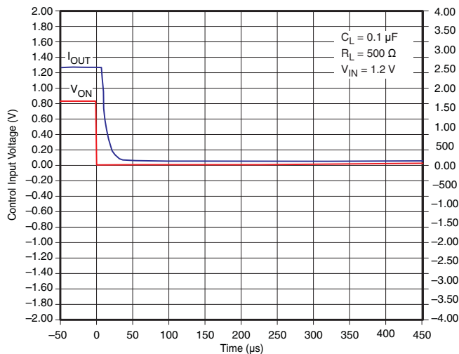
Figure 38. t_{OFF} Response
