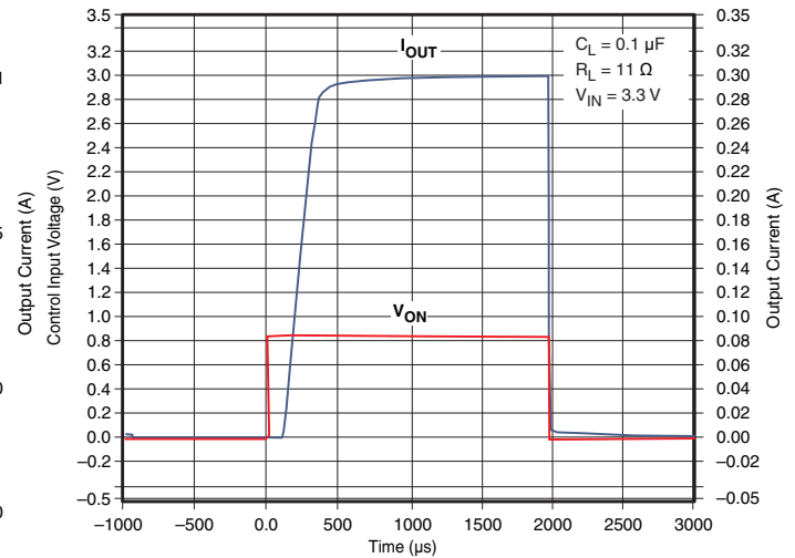
Figure 43. t_{ON} Response
