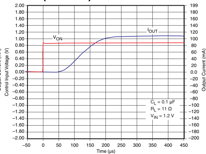
Figure 23. t_{ON} Response
