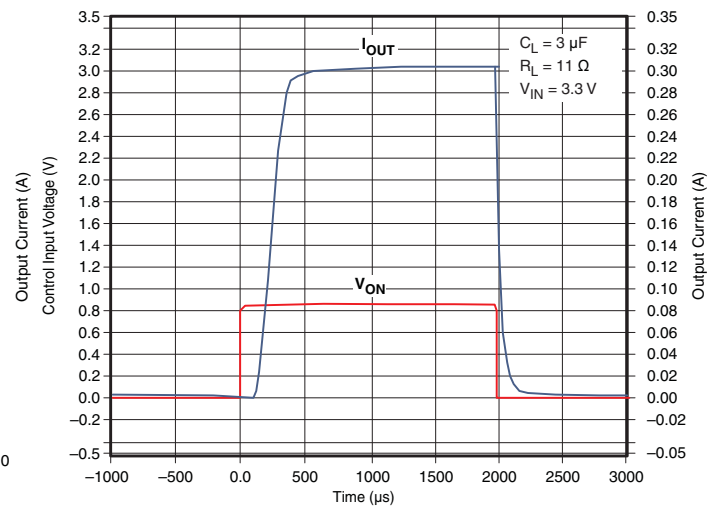
Figure 45. t_{ON} Response
