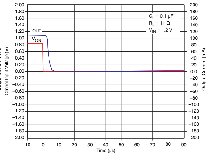
Figure 39. t_{OFF} Response
