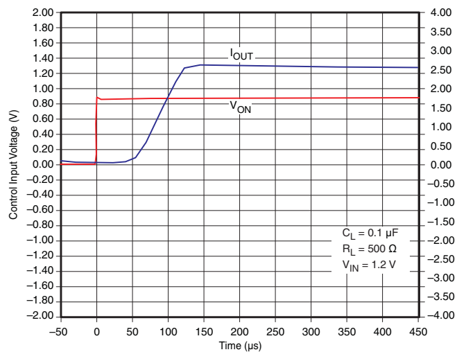
Figure 22. t_{ON} Response
