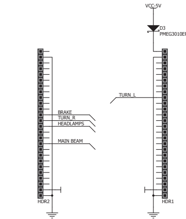
Pins for controlling Buggy's light
