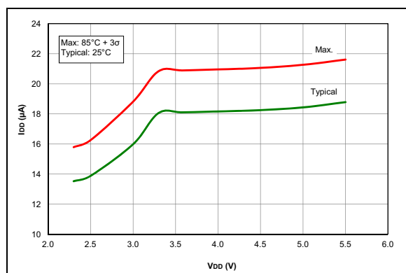
FIGURE 35-8: I_{DD} , EC Oscillator LP Mode, F_{osc} = 32\text{ kHz} , PIC16F1717/8/9 Only.
