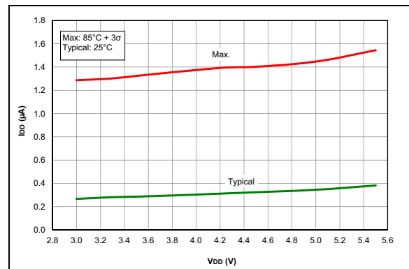
FIGURE 35-42: I_{D, \text{LP Brown-out Reset (LPBOR = 0), PIC16F1717/8/9 Only.}
