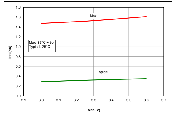
FIGURE 35-41: I_{D, \text{LP Brown-out Reset (LPBOR = 0), PIC16LF1717/8/9 Only.}
