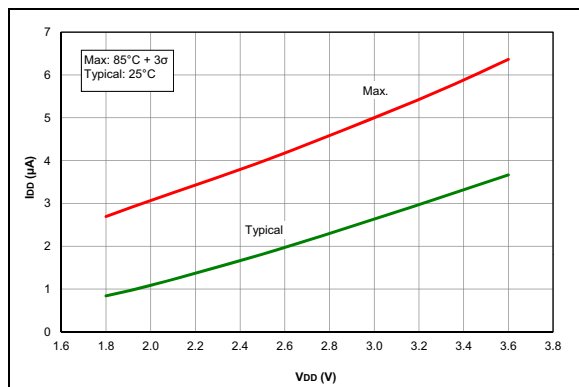
FIGURE 35-43: I_D , Timer1 Oscillator, F_{OSC} = 32\text{ kHz} , PIC16LF1717/8/9 Only.
