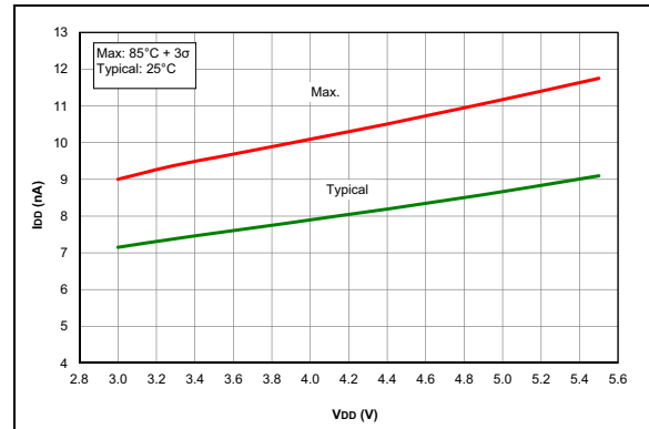
FIGURE 35-40: I_{D, \text{Brown-out Reset (BOR), BORV = 1, PIC16F1717/8/9 Only.}
