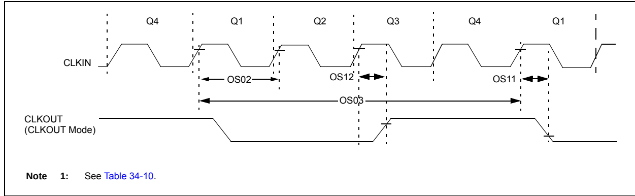
FIGURE 34-5: CLOCK TIMING
