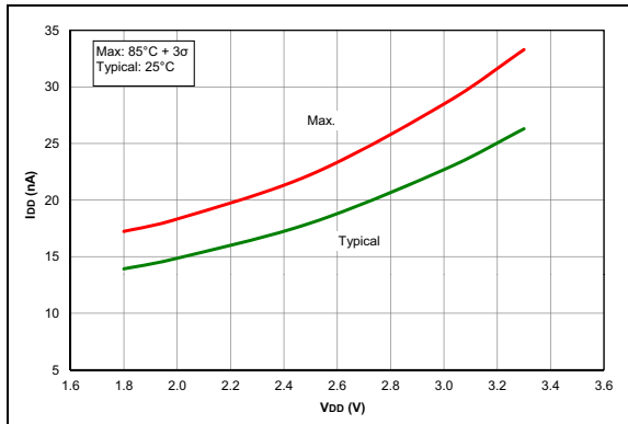
FIGURE 35-37: I_{D, \text{Fixed Voltage Reference (FVR), PIC16LF1717/8/9 Only.}
