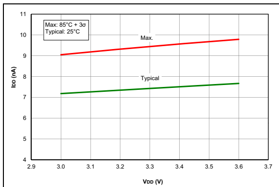
FIGURE 35-39: I_{D, \text{Brown-out Reset (BOR), BORV = 1, PIC16LF1717/8/9 Only.}
