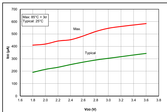
FIGURE 35-45: I_D , Op Amp, High GBWP Mode ( OPAxSP = 1 ), PIC16LF1717/8/9 Only.
