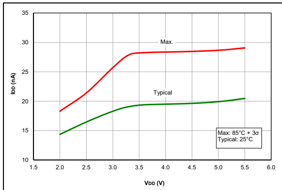
FIGURE 35-38: I_{D, \text{Fixed Voltage Reference (FVR), PIC16F1717/8/9 Only.}
