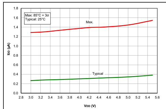
FIGURE 35-42: I_{DD} , LP Brown-out Reset (LPBOR = 0), PIC16F1717/8/9 Only.
