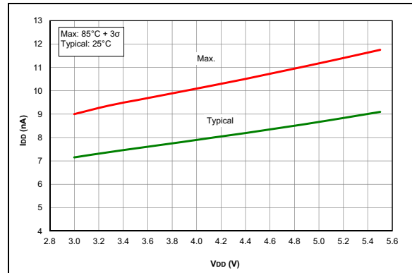
FIGURE 35-40: I_{DD} , Brown-out Reset (BOR), BORV = 1, PIC16F1717/8/9 Only.
