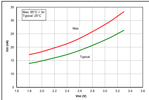
FIGURE 35-37: I_{DD} , Fixed Voltage Reference (FVR), PIC16LF1717/8/9 Only.
