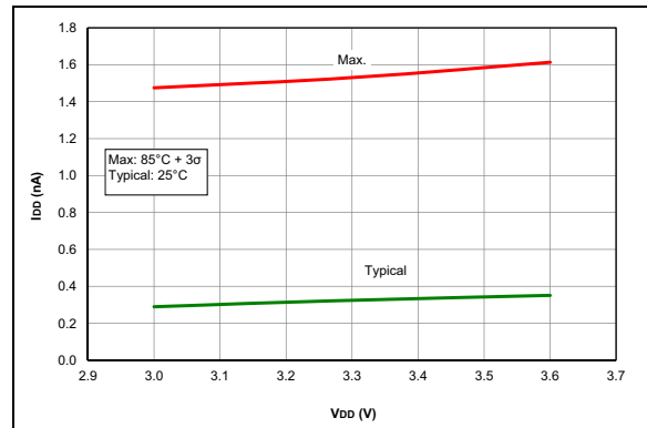
FIGURE 35-41: I_{DD} , LP Brown-out Reset (LPBOR = 0), PIC16LF1717/8/9 Only.
