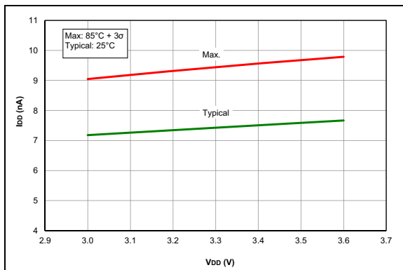
FIGURE 35-39: I_{DD} , Brown-out Reset (BOR), BORV = 1, PIC16LF1717/8/9 Only.
