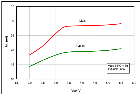
FIGURE 35-38: I_{DD} , Fixed Voltage Reference (FVR), PIC16F1717/8/9 Only.
