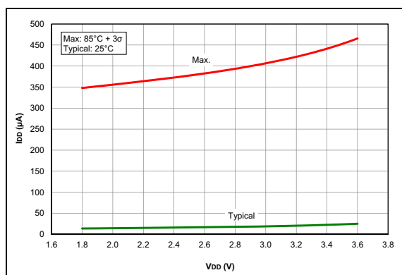
FIGURE 35-47: I_D , ADC Non-Converting, PIC16LF1717/8/9 Only.
