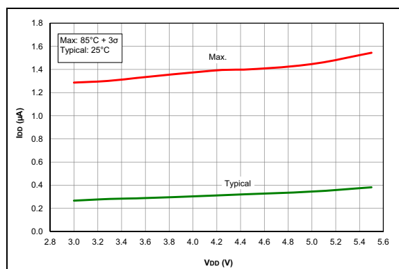
FIGURE 35-42: I_{D} , LP Brown-out Reset (LPBOR = 0), PIC16F1717/8/9 Only.
