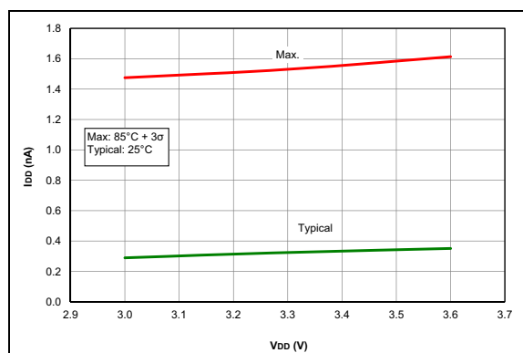
FIGURE 35-41: I_{D} , LP Brown-out Reset (LPBOR = 0), PIC16LF1717/8/9 Only.
