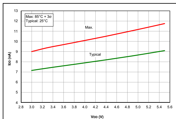
FIGURE 35-40: I_{D} , Brown-out Reset (BOR), BORV = 1, PIC16F1717/8/9 Only.
