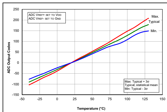
FIGURE 35-89: Temp. Indicator Slope Normalized to 20^\circ C , High Range, V_{DD} = 3.0V , PIC16F1717/8/9 Only.
