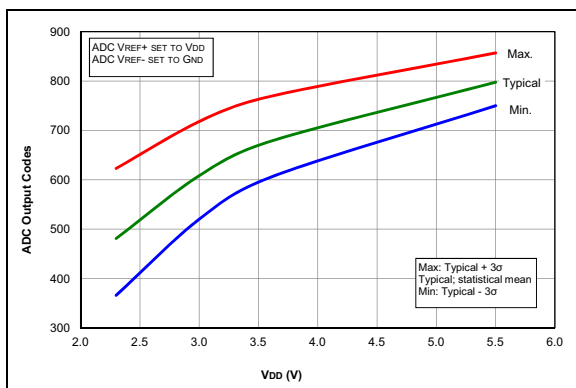
FIGURE 35-86: Temp. Indicator Initial Offset, Low Range, Temp. = 20^\circ C , PIC16F1717/8/9 Only.
