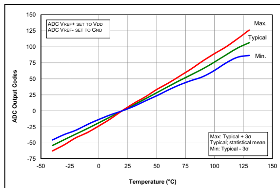
FIGURE 35-90: Temp. Indicator Slope Normalized to 20^\circ C , Low Range, V_{DD} = 3.0V , PIC16F1717/8/9 Only.
