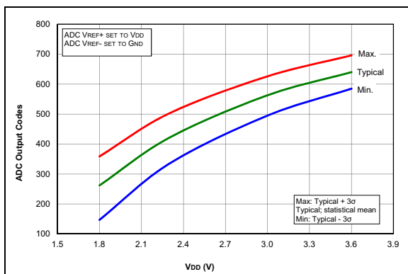
FIGURE 35-87: Temp. Indicator Initial Offset, Low Range, Temp. = 20^\circ C , PIC16LF1717/8/9 Only.
