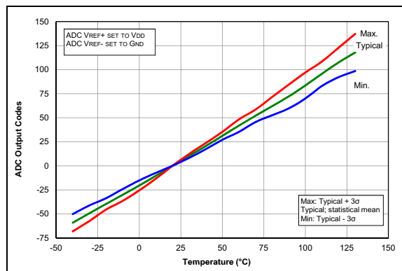
FIGURE 35-88: Temp. Indicator Slope Normalized to 20^\circ C , High Range, V_{DD} = 5.5V , PIC16F1717/8/9 Only.
