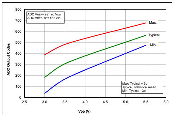
FIGURE 35-85: Temp. Indicator Initial Offset, High Range, Temp. = 20^\circ C , PIC16F1717/8/9 Only.
