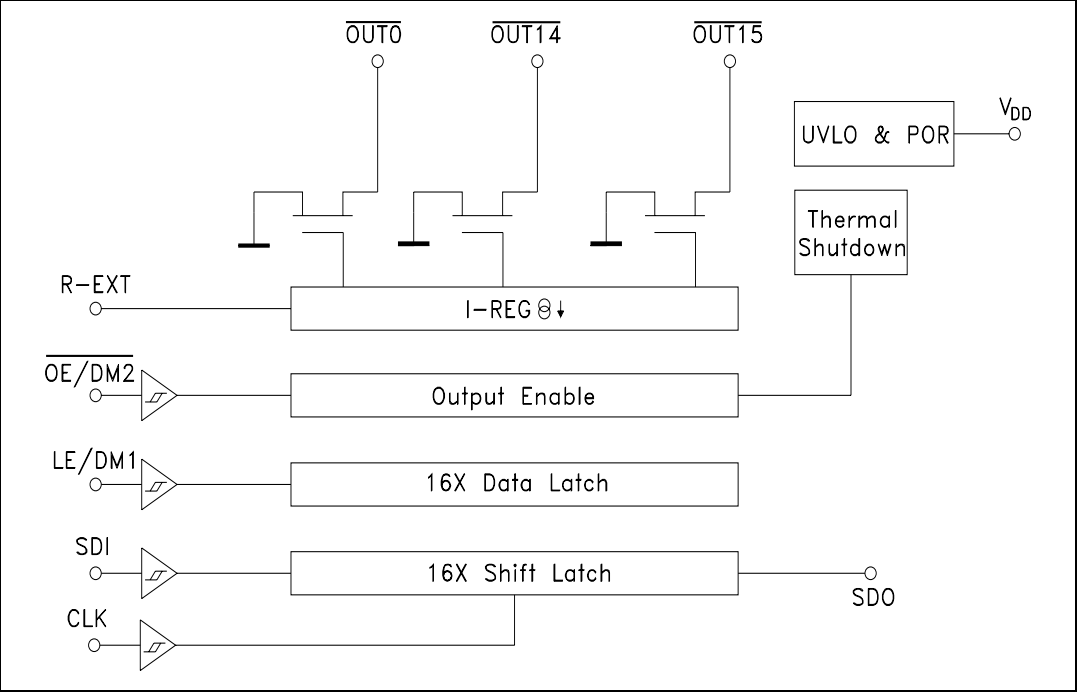
Figure 7. Block diagram
