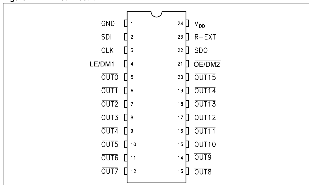
Figure 2. Pin connection
