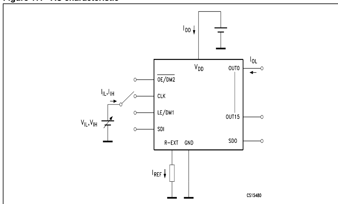
Figure 17. AC characteristic
