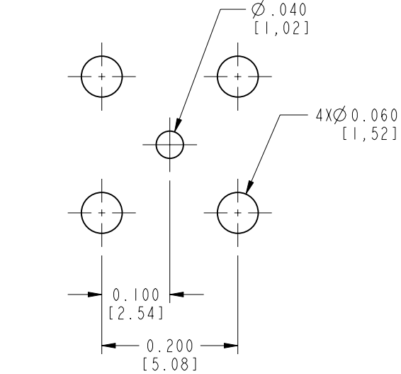
RECOMMENDED PCB MOUNTING DIMENSIONS
