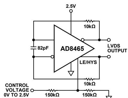
Figure 23. Voltage-Controlled Oscillator
