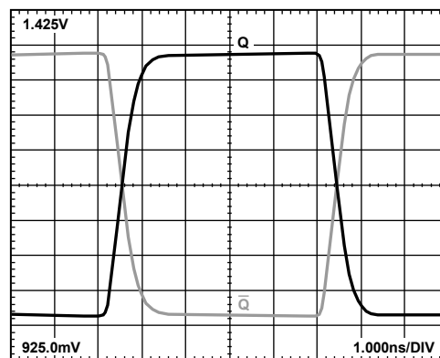
Figure 14. 50 MHz Output Voltage Waveform at V_{CCO} = 2.5\text{ V}
