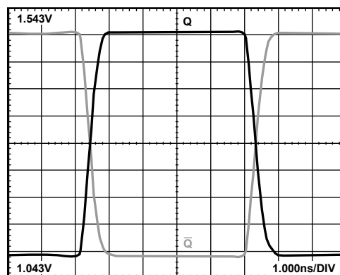
Figure 15. 50 MHz Output Voltage Waveform at V_{CCO} = 5.5\text{ V}
