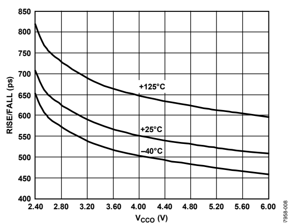
Figure 8. LVDS Output Rise/Fall Time vs. V_{CC0}
