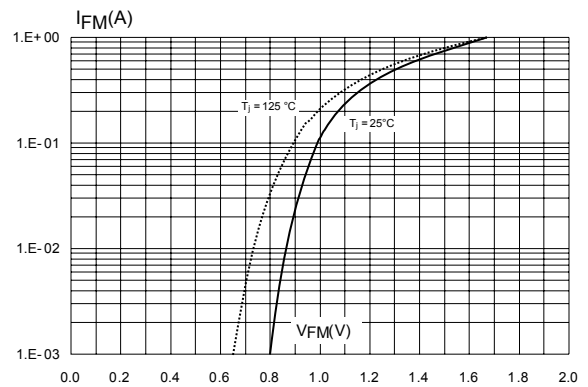
Figure 5. Forward voltage drop versus peak forward current
