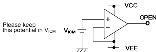
Figure 117. Disable Circuit Example
