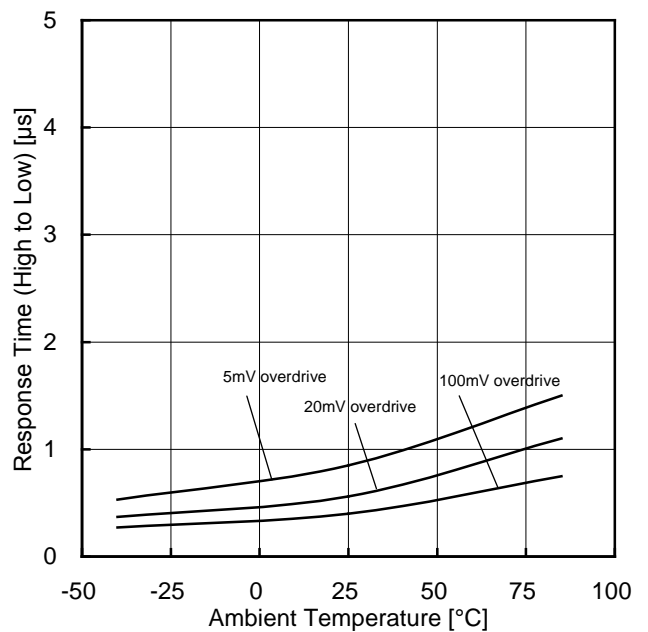
Figure 64. Response Time (High to Low) vs Ambient Temperature (VCC=5V, V RL =5V, R L =5.1kΩ)
