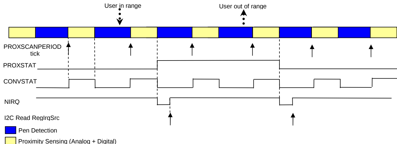
Figure 42 – Proximity Sensing Host Operation (Pen Trigger Mode ; ReglqMsk[6:4] = 110 ; PROXIRQSEL = 0 )
