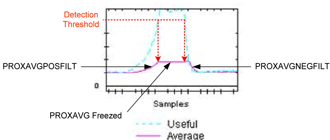
Figure 38 – ProxAvg vs Proximity Event
