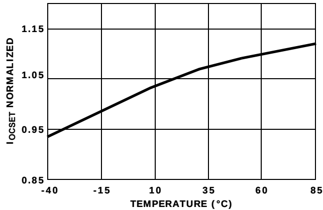
FIGURE 3. IOCSSET vs TEMPERATURE
