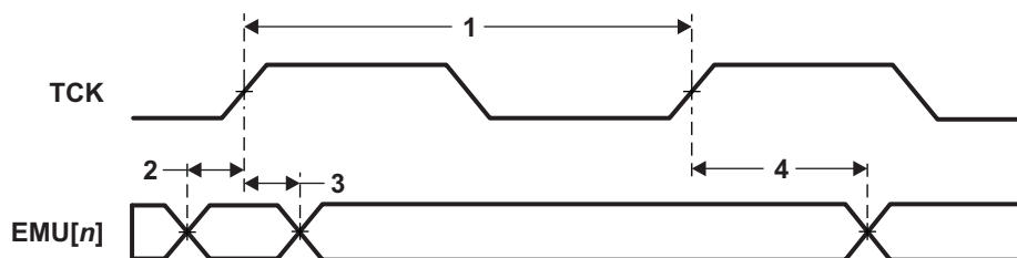
Figure 7-47. HS-RTDX Timing
