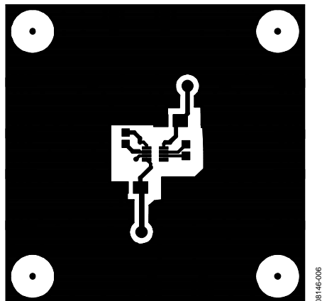
Figure 5. Evaluation Board Layout Pattern, Component Side
