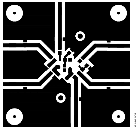
Figure 7. Evaluation Board Layout Pattern, Circuit Side
