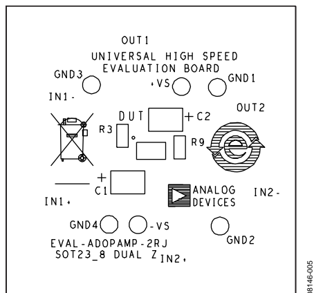
Figure 4. Evaluation Board Assembly Drawing, Component Side
