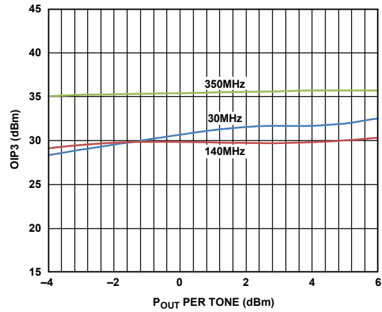
Figure 12. OIP3 vs. Output Power ( P_{OUT} ) and Frequency, Low Frequency Configuration
