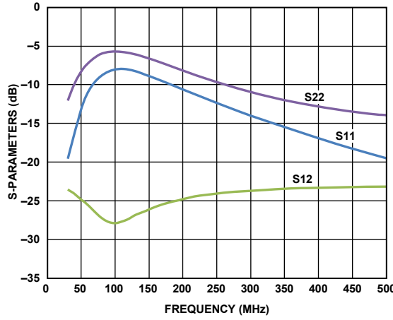
Figure 13. Output Return Loss (S22), Input Return Loss (S11), and Reverse Isolation (S12) vs. Frequency, Low Frequency Configuration
