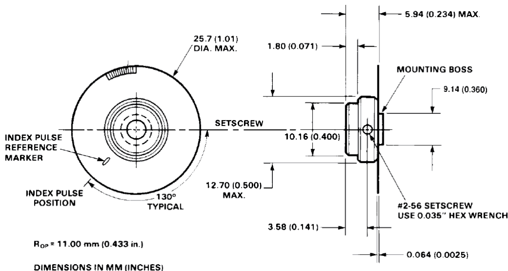
Figure 6. HED5-5140 Codewheel Used with HEDT-9140.
