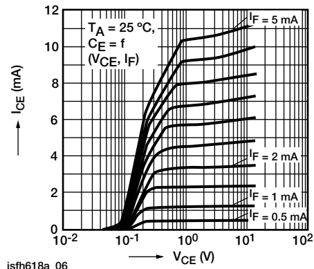
Fig. 9 - Output Characteristics
