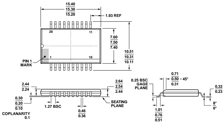
COMPLIANT TO JEDEC STANDARDS MS-013 Figure 59. 20-Lead Standard Small Outline Package, with Increased Creepage [SOIC_IC] Wide Body (RI-20-1) Dimensions shown in millimeters
