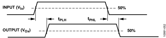
Figure 52. Propagation Delay Parameters
