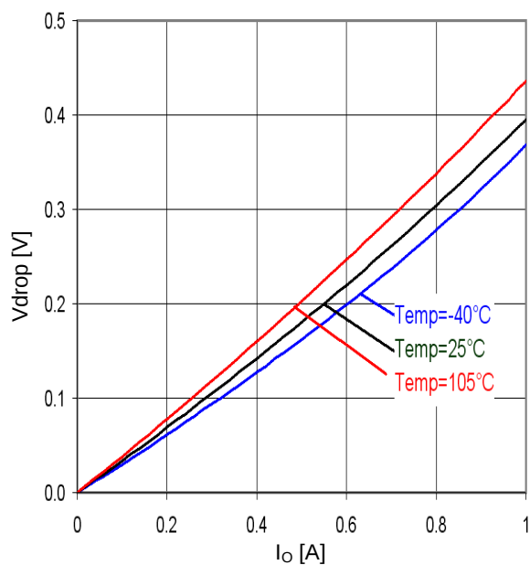
Figure 37. Minimum dropout Voltage 5 (V CC =5.5V, Ta=25°C)
