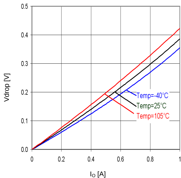
Figure 36. Minimum dropout Voltage 2 (V CC =4V, Ta=25°C)
