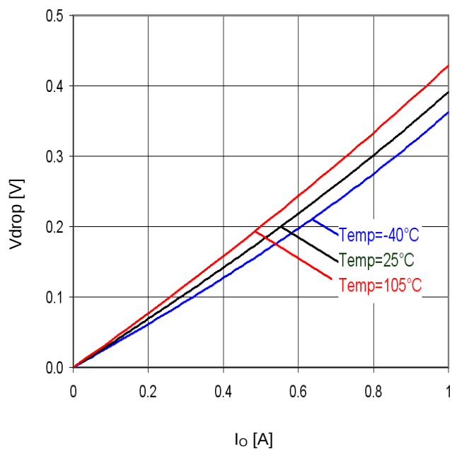
Figure 35. Minimum dropout Voltage 2 (V CC =3.3, Ta=25°C)
