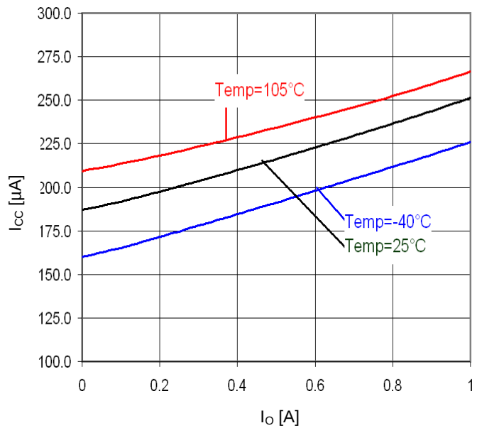
Figure 32. I_o - I_{cc}
