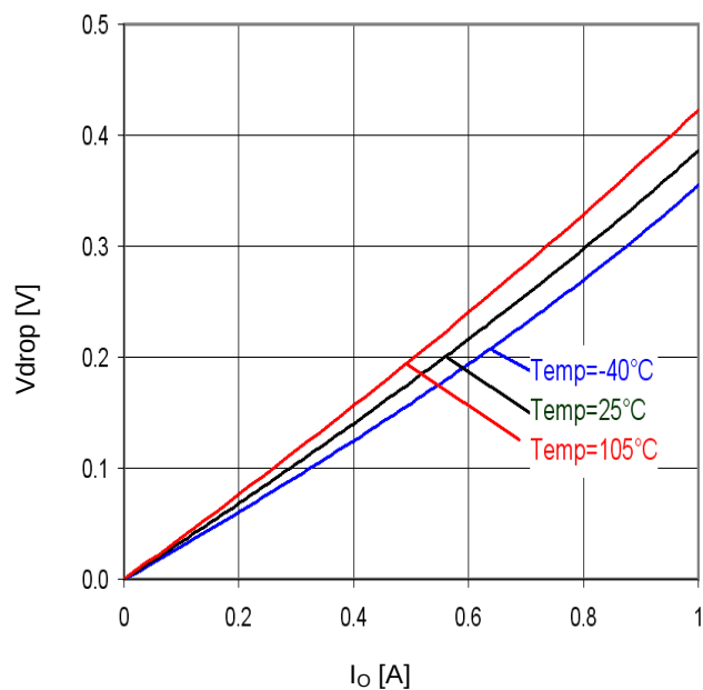
Figure 36. Minimum dropout Voltage 2 ( V_{CC}=4 , T_a=25^\circ\text{C} )
