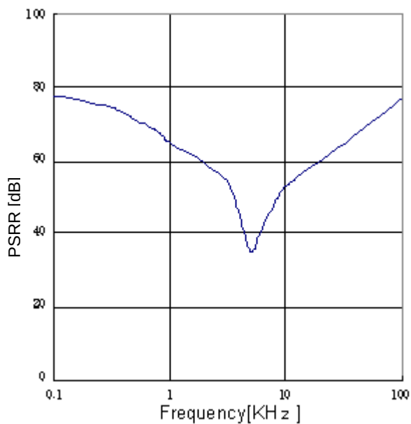
Figure 33. PSRR ( I_o=0 mA)
