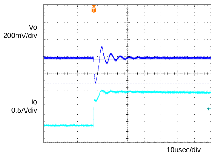
Figure 5. Transient Response (0→1.0A) C_o=1\mu F , T_a=105^\circ C
