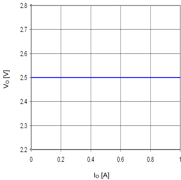
Figure 25. I_O - V_O
