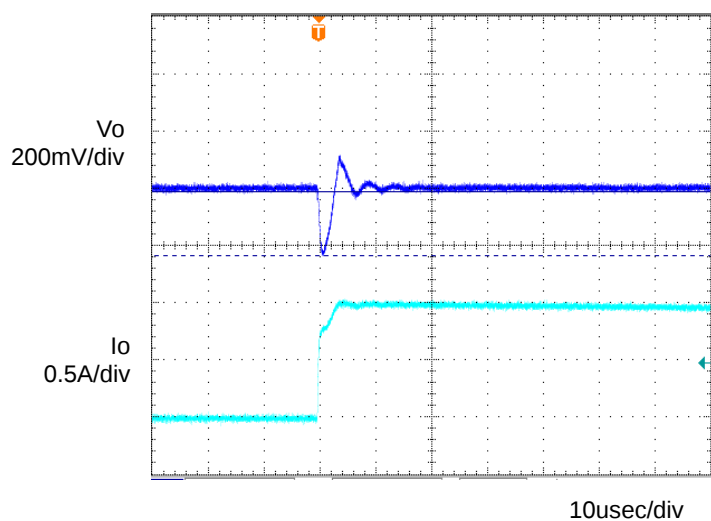
Figure 3. Transient Response (0→1.0A) C_o=1\mu F , T_a=-40^\circ C
