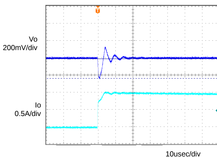
Figure 4. Transient Response (1.0→0A) C_o=1\mu F , T_a=25^\circ C
