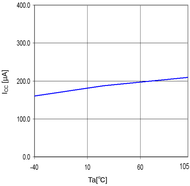
Figure 22. T_a - I_{CC}
