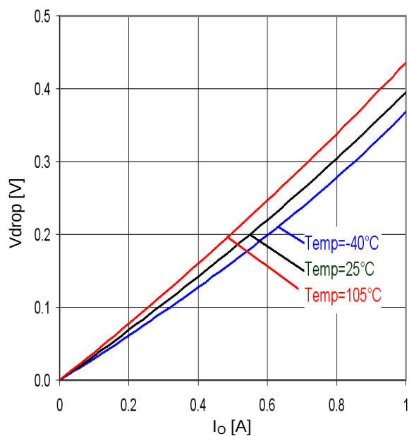
Figure 37. Minimum dropout Voltage 5 ( V_{CC}=5.5 , T_a=25^\circ\text{C} )
