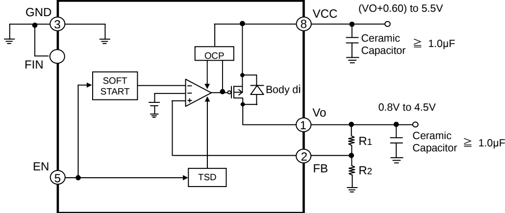
Figure 1. Block Diagram
