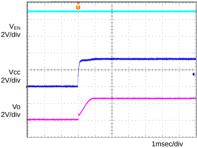
Figure 9. Input sequence 1 C_o=1\mu\text{F} , T_a=-40^\circ\text{C}
