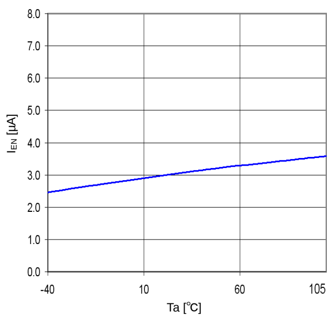
Figure 24. T_a - I_{EN}
