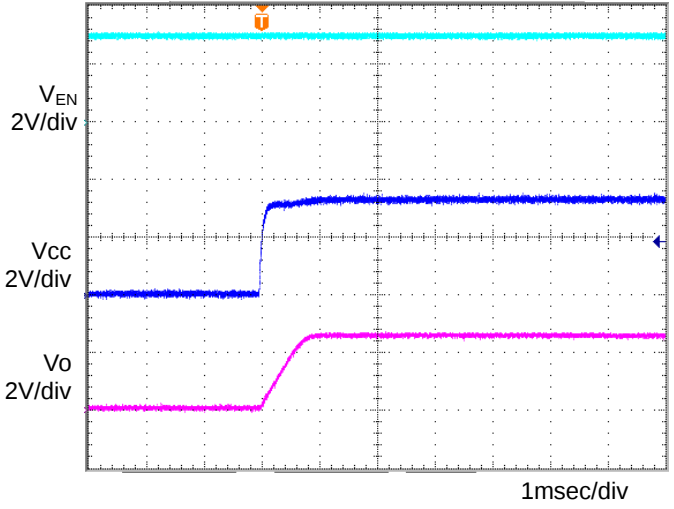
Figure 10. Input sequence 1 C_o=1\mu\text{F} , T_a=25^\circ\text{C}
