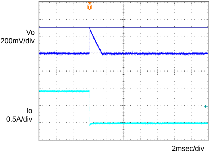
Figure 7. Transient Response (1.0→0A) C_o=1\mu\text{F} , T_a=25^\circ\text{C}
