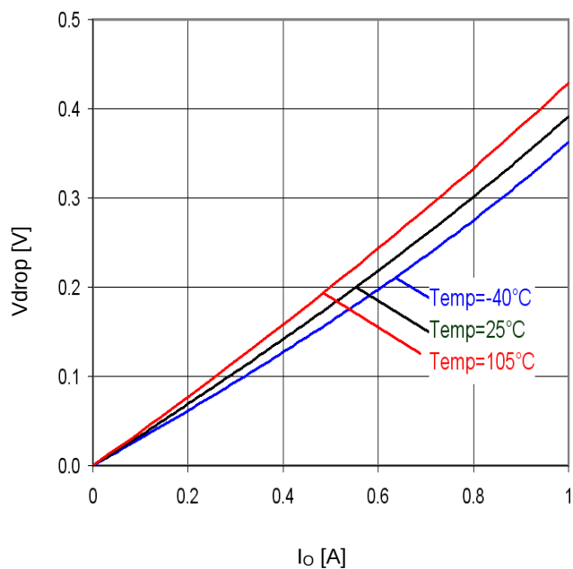
Figure 35. Minimum dropout Voltage 2 ( V_{CC}=3.3 , T_a=25^\circ\text{C} )
