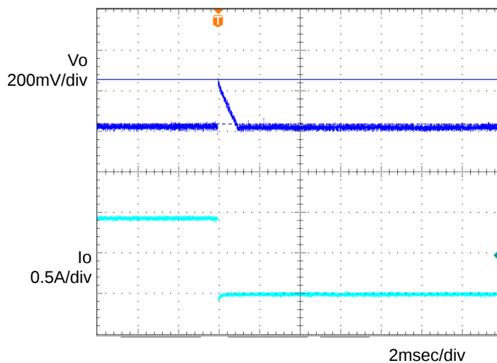
Figure 6. Transient Response (1.0→0A) C_o=1\mu F , T_a=-40^\circ C
