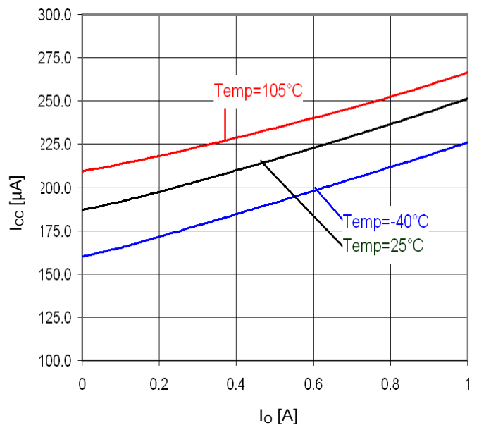
Figure 32. I_o - I_{cc}
