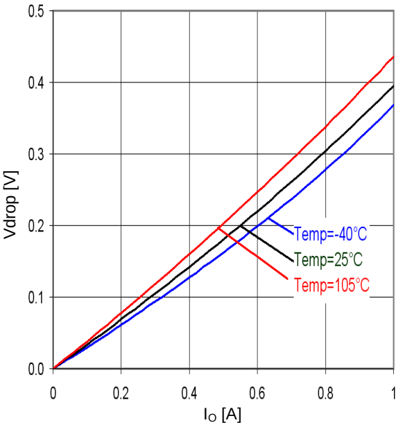
Figure 37. Minimum dropout Voltage 5 (V CC =5.5V, Ta=25°C)
