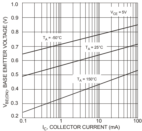
Fig. 5 Base-Emitter Voltage vs. Collector Current
