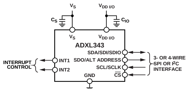
Figure 34. Application Diagram
