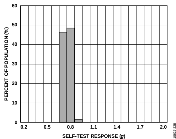
Figure 19. X-Axis Self-Test Response at 25^\circ\text{C} , V_S = 2.5\text{ V}
