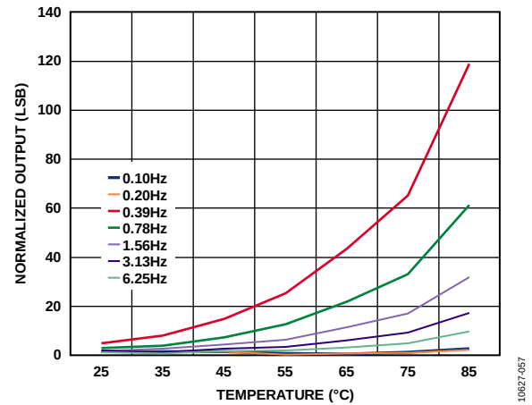
Figure 45. Typical Y-Axis Output vs. Temperature at Lower Data Rates, Normalized to 100 Hz Output Data Rate, V_S = 2.5 V
