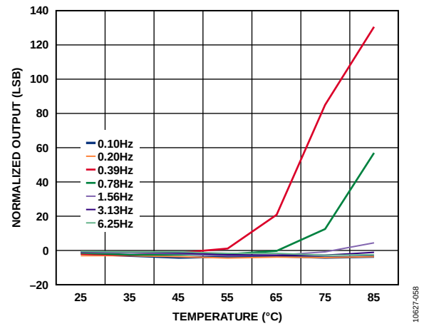
Figure 46. Typical Z-Axis Output vs. Temperature at Lower Data Rates, Normalized to 100 Hz Output Data Rate, V_S = 2.5 V
