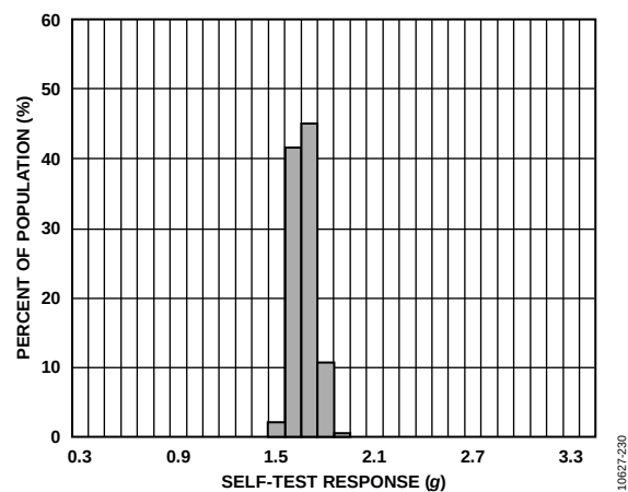
Figure 21. Z-Axis Self-Test Response at 25^\circ\text{C} , V_S = 2.5\text{ V}
