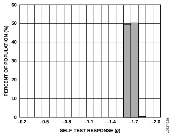
Figure 20. Y-Axis Self-Test Response at 25^\circ\text{C} , V_S = 2.5\text{ V}
