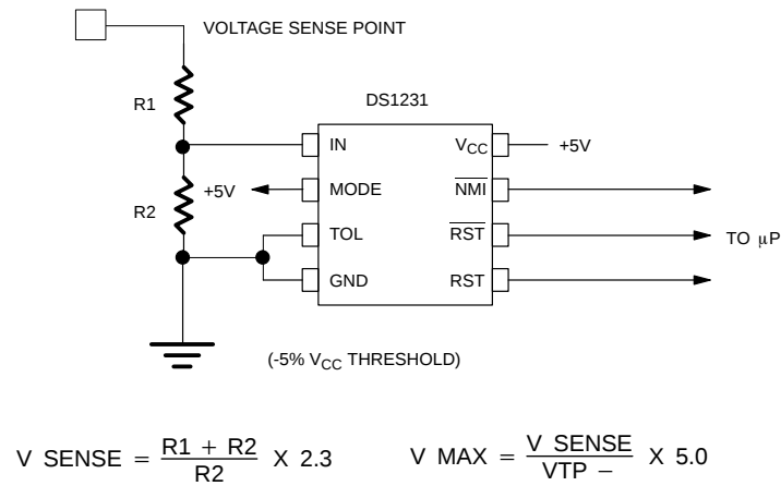
APPLICATION WITH MODE PIN CONNECTED TO V CC Figure 4
