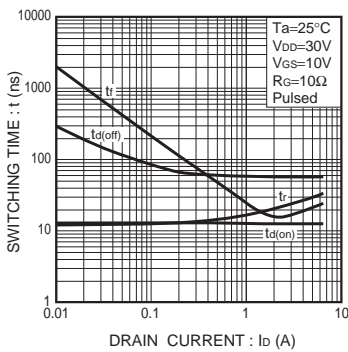
Fig.7 Switching Characteristics
