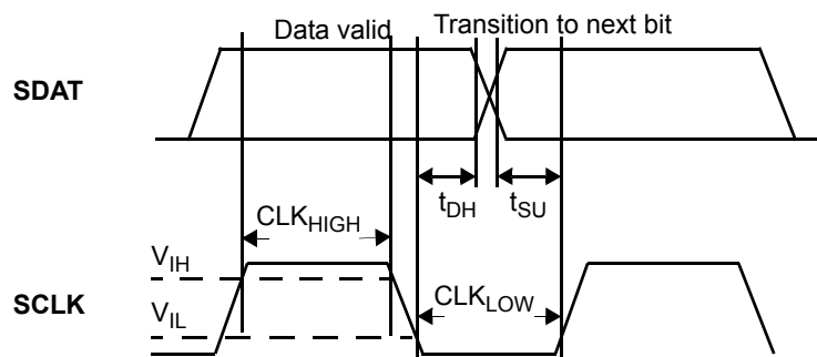
Figure 2. Data Valid and Data Transition Periods
