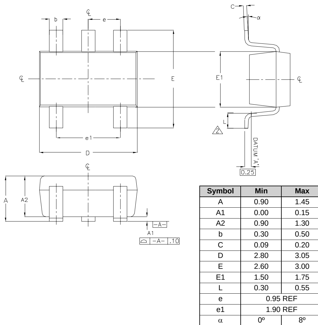
Figure 18. 5-pin SOT23 Package
