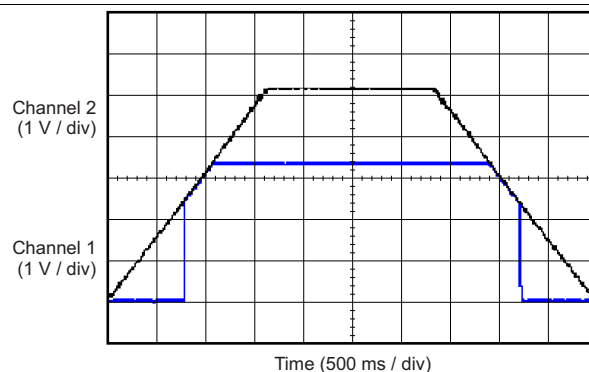
Figure 38. TPS70933-Q1 Line Transient (4.3 V to 5.3 V)
