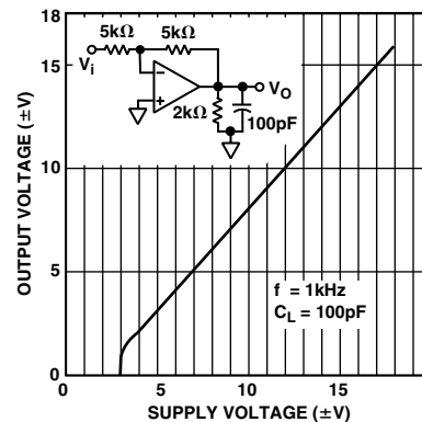
TPC 3. Output Voltage Swing vs. Supply Voltage
