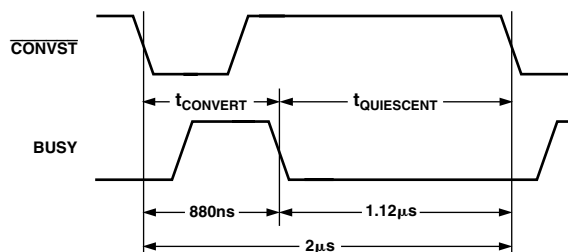
Figure 12. Mode 1 Power Dissipation
