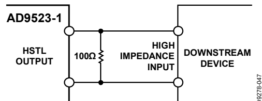
Figure 22. DC-Coupled HSTL Output Driver
