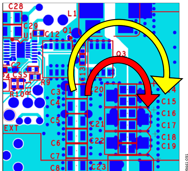
Figure 91. Primary Current Pathways During the On State of the High-Side MOSFET (Left Arrow) and the On State of the Low-Side MOSFET (Right Arrow)
