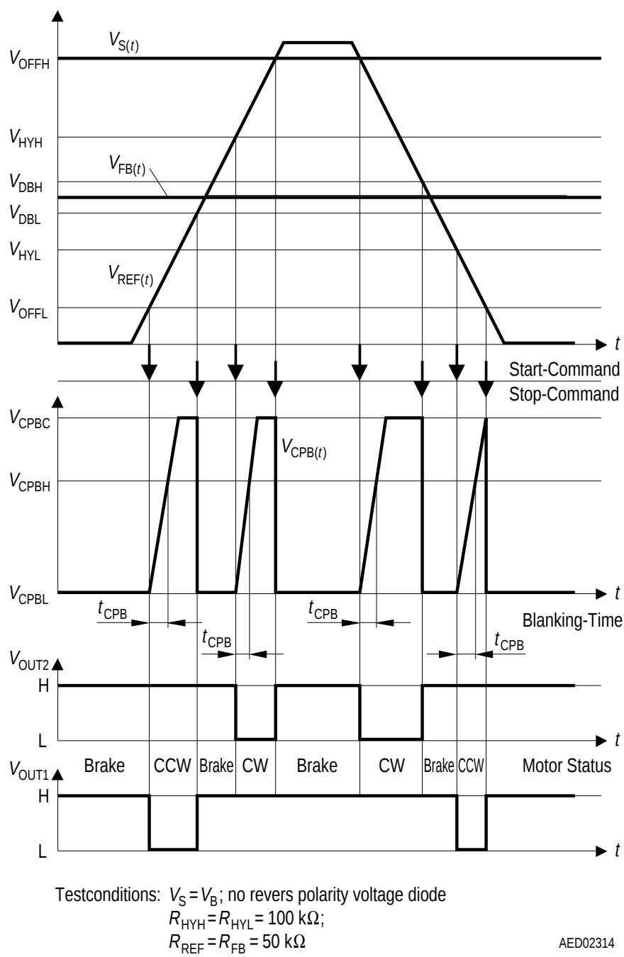
Figure 5 Timing and Phaselag
