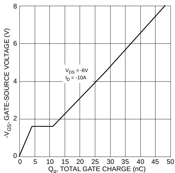
Figure 10 Gate-Charge Characteristics
