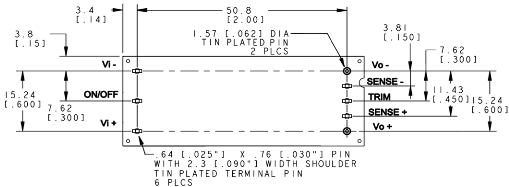
Bottom View
