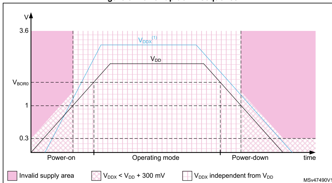
Figure 3. Power-up/down sequence
