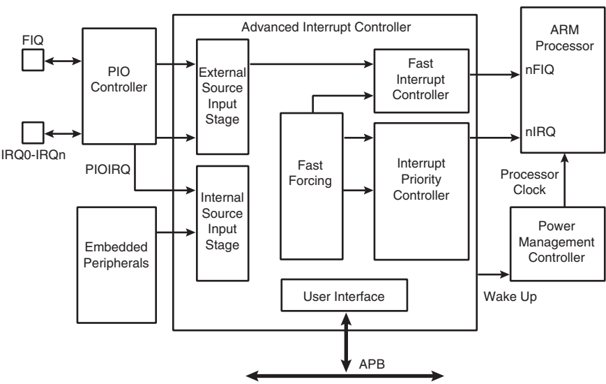
Figure 27-3. AIC Detailed Block Diagram
