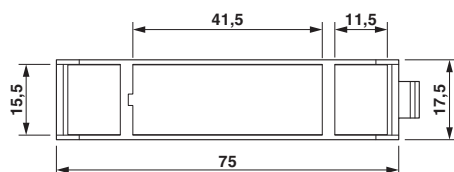
Dimensional drawing
