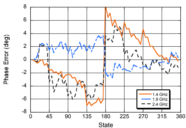
Phase Error (degrees) vs. State
