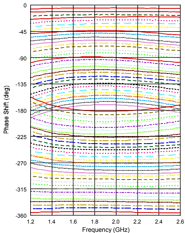
Phase Shift vs. Frequency (All States)
