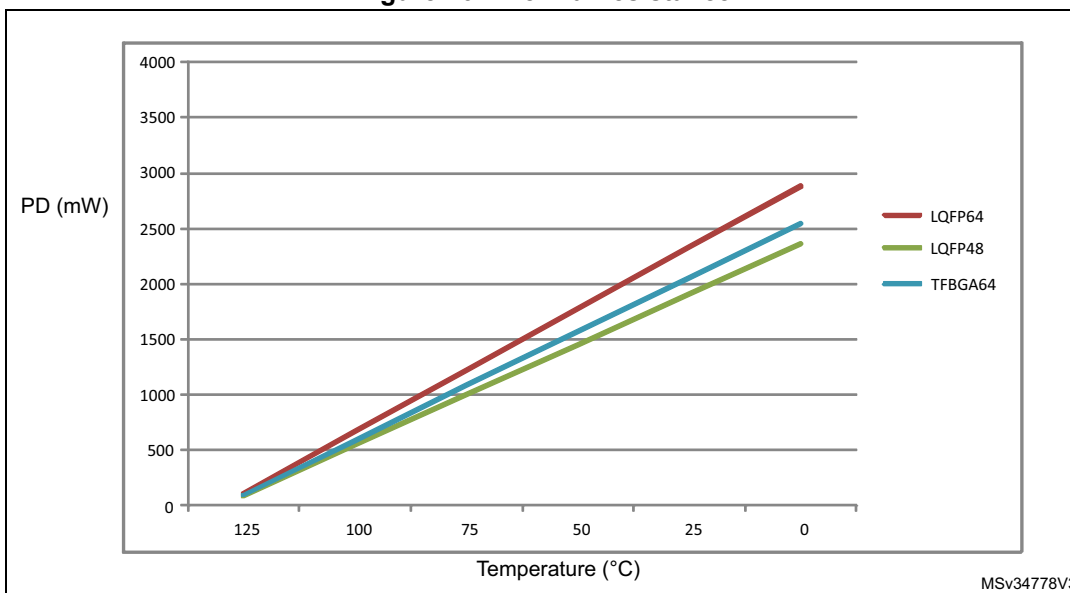
Figure 46. Thermal resistance
